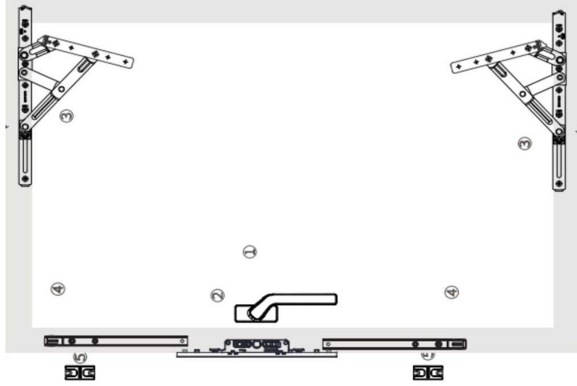
Outward Opening Glass window Solution
